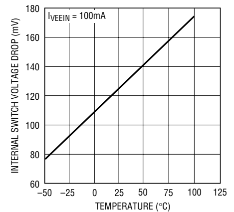
V_{\text{EE}} Internal Switch Voltage Drop vs Temperature
