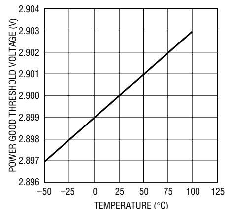
Power Good Threshold Voltage vs Temperature ( 3V_{\text{OUT}} )
