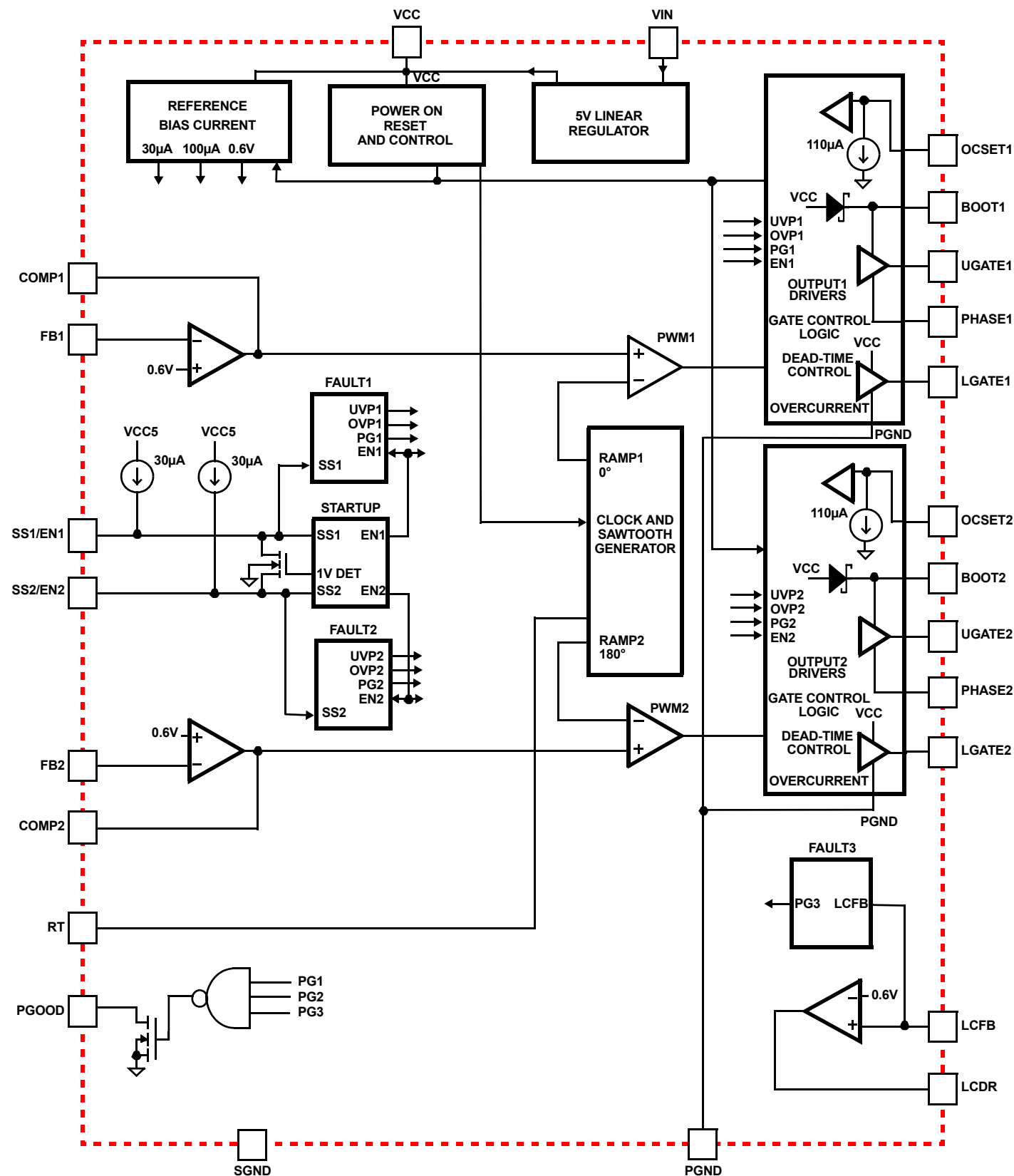
FIGURE 1. BLOCK DIAGRAM
