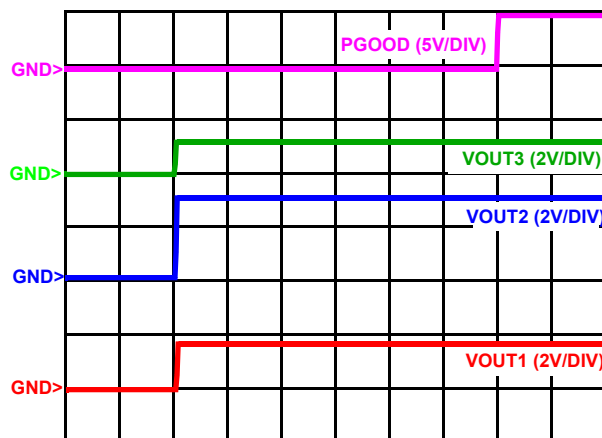
FIGURE 9. PGOOD DELAY
