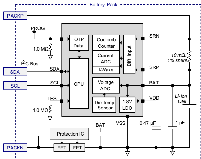
Simplified Schematic
