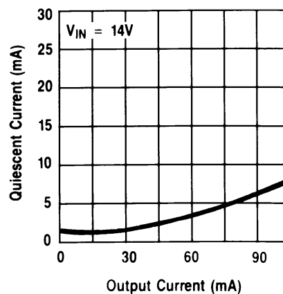
Quiescent Current
