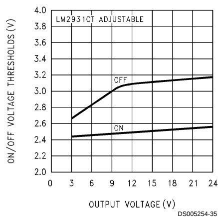
On/Off Threshold
