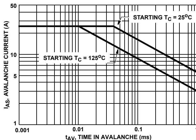
FIGURE 2. UNCLAMPED INDUCTIVE-SWITCHING
