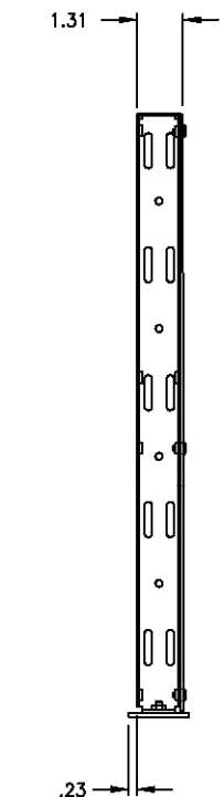
SECTION Z-Z
