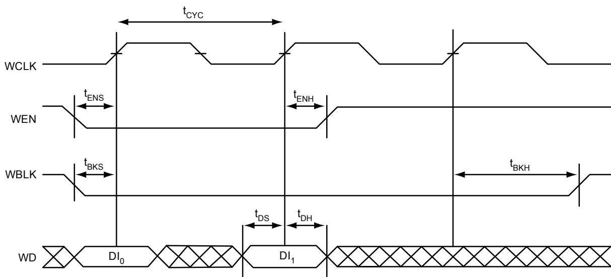
Figure 2-48 • FIFO Write
