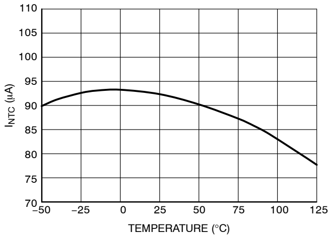
Figure 17. Current I NTC Sourced from the Latch Pin, Allowing Direct NTC Connection
