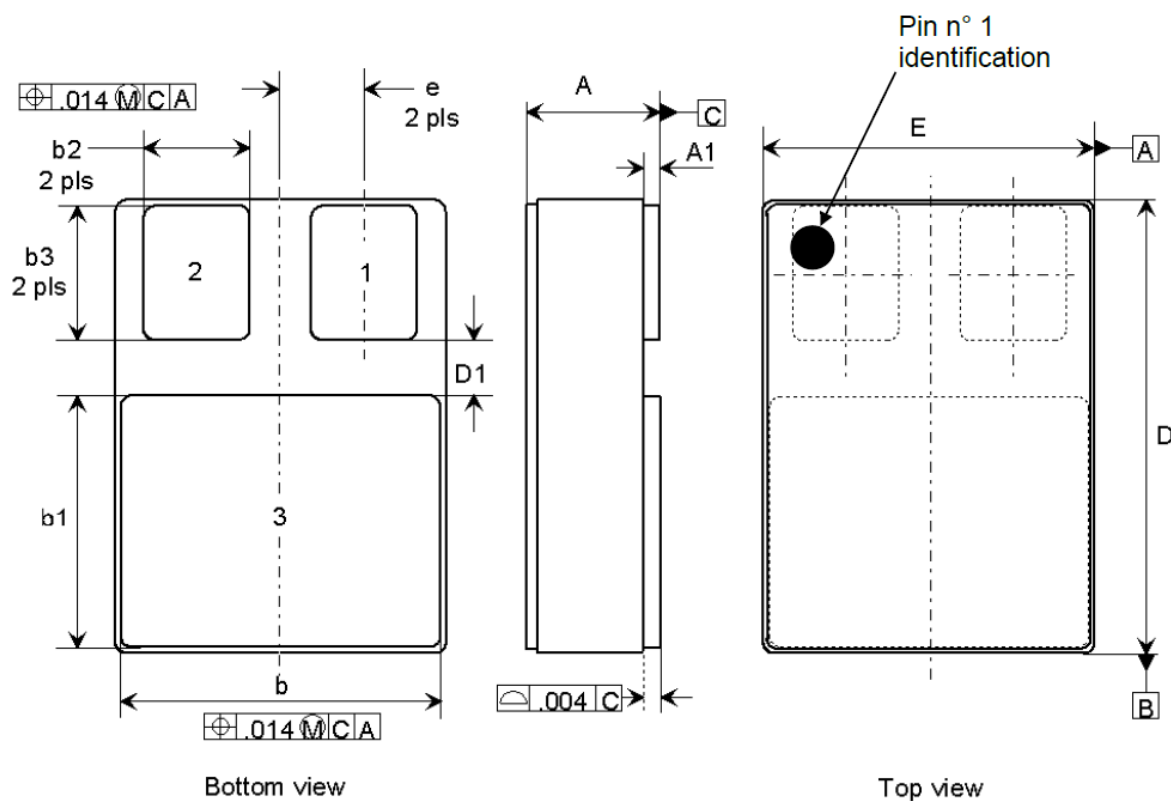
Figure 7. SMD.5 package outline
