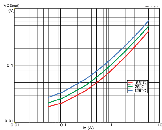
Figure 2. V_{CE(sat)} at h_{FE} = 10
