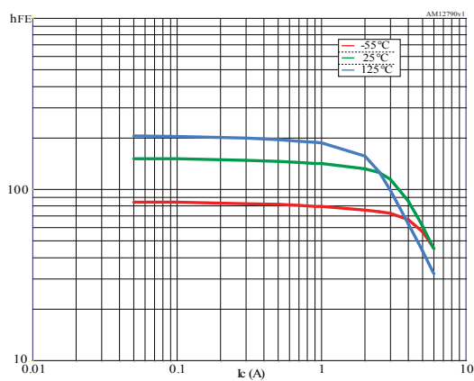
Figure 1. h_{FE} at V_{CE} = 5\text{ V}
