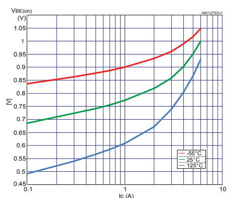
Figure 4. V_{BE(on)} at V_{CE} = 5\text{ V}
