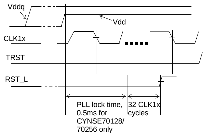
Figure 13-2. Alternative Power-up Sequence (CLK1x)
