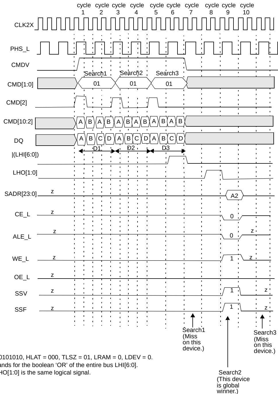
Figure 10-54. Timing Diagram for 288-bit Search Device Number 1
