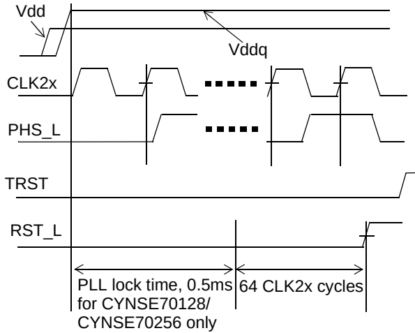
Figure 13-3. Proper Power-up Sequence (CLK2x)
