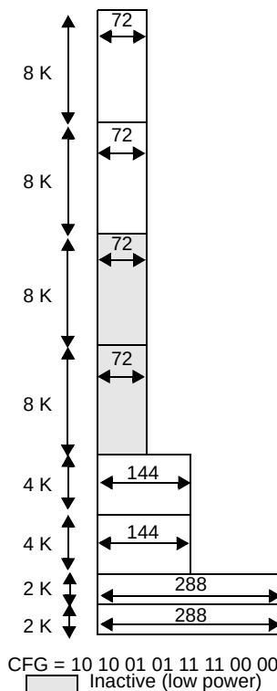
Figure 8-2. Multiwidth Database Configurations Example
