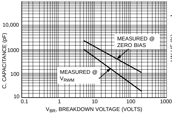
Figure 3. Capacitance versus Breakdown Voltage
