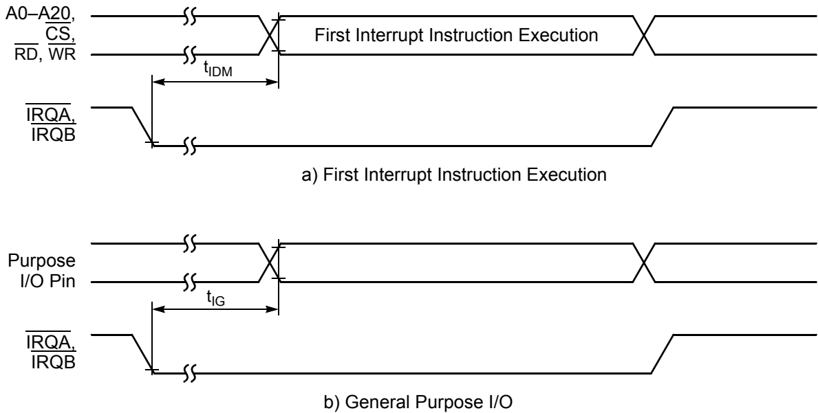
Figure 4-13 External Level-Sensitive Interrupt Timing
