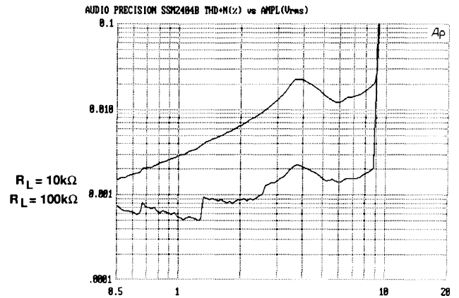
Figure 2. Headroom ( V_S = \pm 12\text{ V} , f = 1\text{ kHz} , with 80 kHz Filter)
