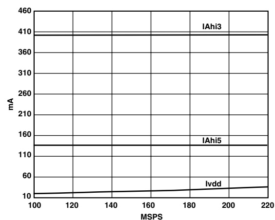
TPC 11. Power Supply Currents vs. Encode
