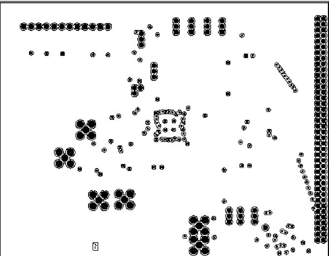
Figure 16. Ground Plane
