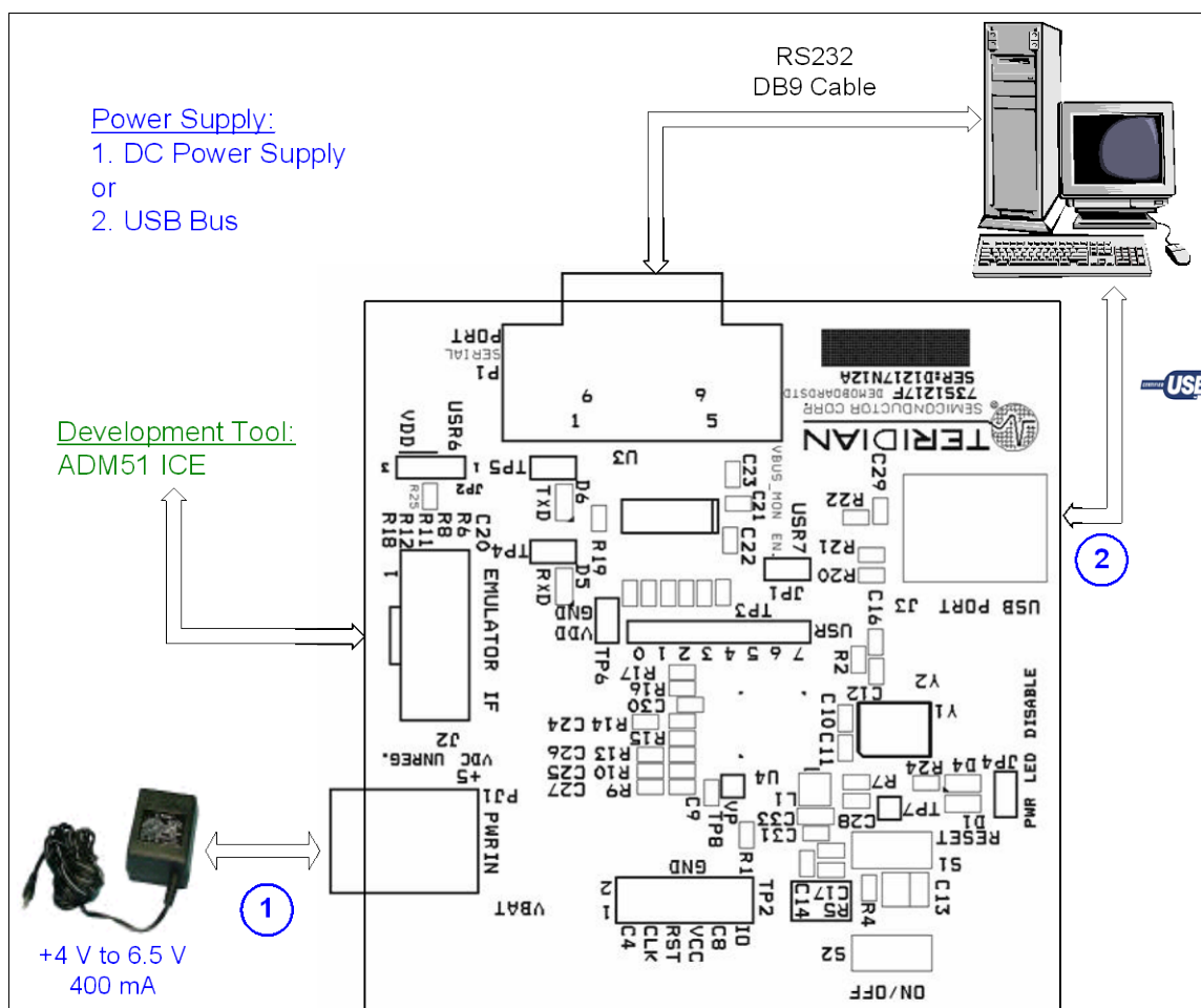
Figure 2: 73S1217F Evaluation Board Lite Basic Connections
