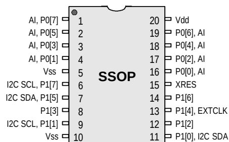
CY8C21334 20-Pin PSoC Device
