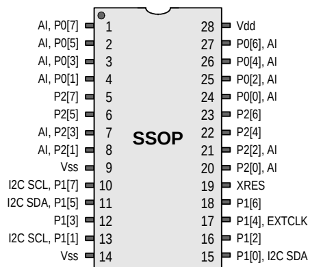
CY8C21534 28-Pin PSoC Device
