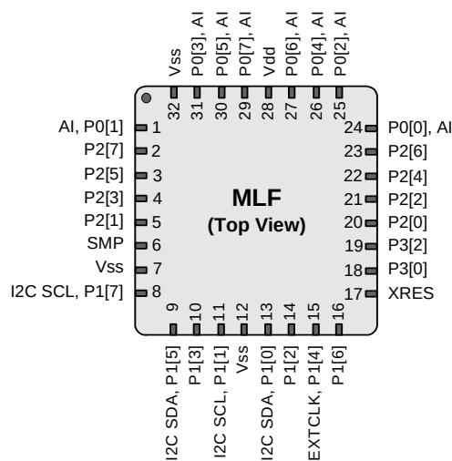
CY8C21634 32-Pin PSoC Device
