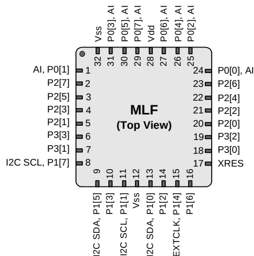
CY8C21434 32-Pin PSoC Device
