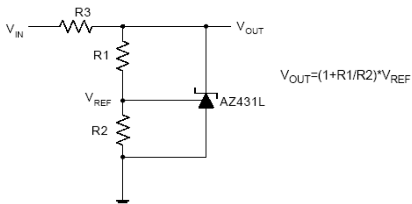
Shunt Regulator
