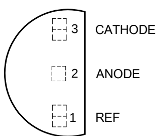
(TO-92 (Ammo Packing)/ Z Package)
