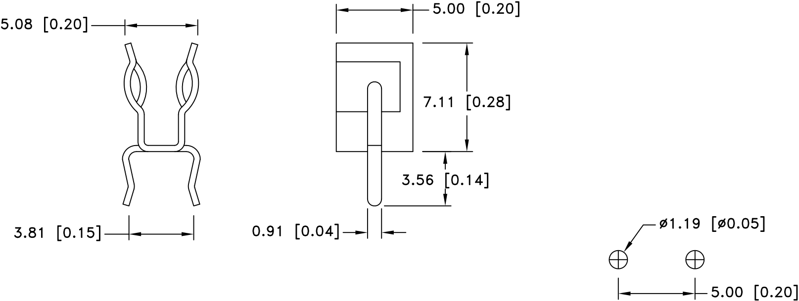
MOUNTING DETAIL
