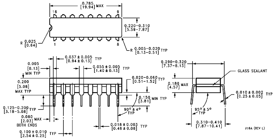
Order Number MM54HC147J or MM74HC147J NS Package J16A
