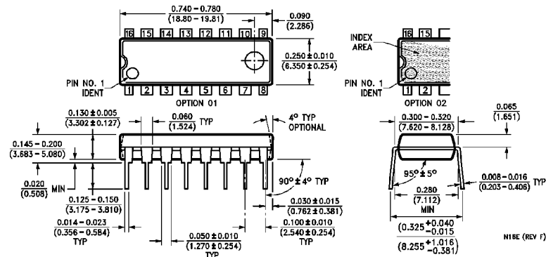
Order Number MM74HC147N NS Package N16E
