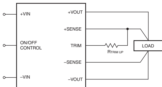
Figure 9. Trim Connections To Increase Output Voltages Using Fixed Resistors
