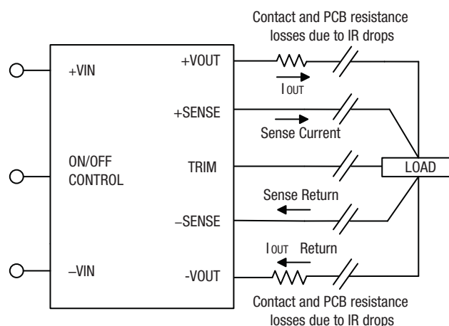
Figure 11. Remote Sense Circuit Configuration
