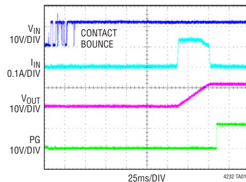
Power-Up Waveforms
