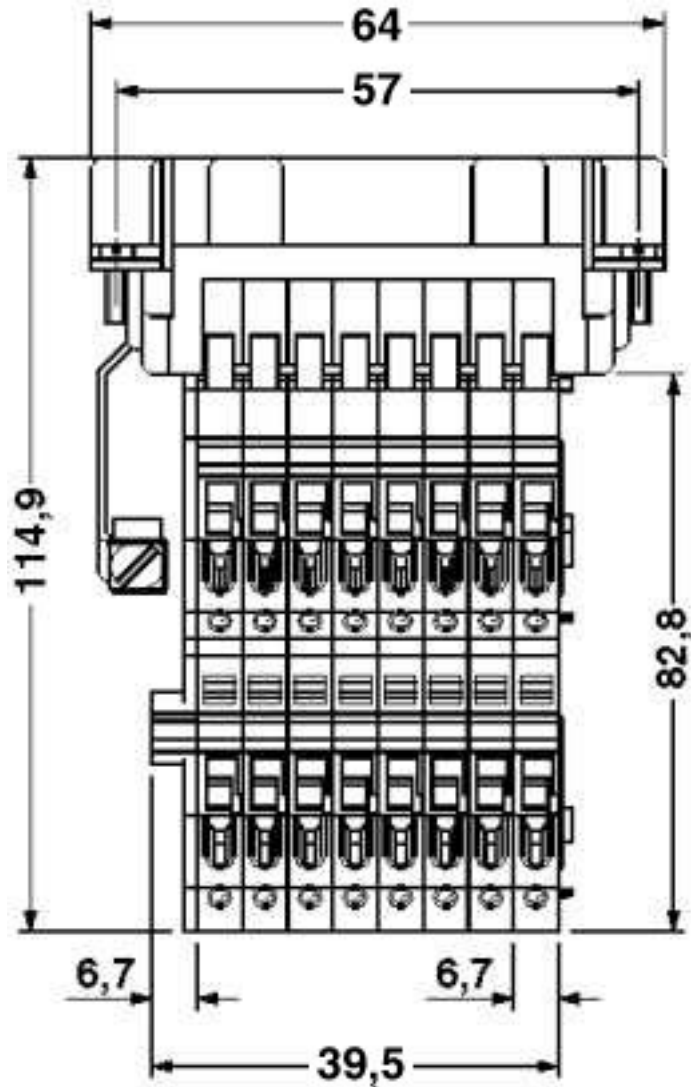
Dimensioned drawing
