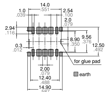
1 coil latching
