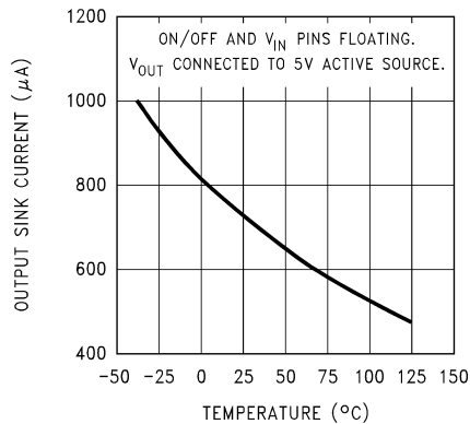
Figure 5-43. Output Reverse Leakage vs Temperature (Legacy Chip)
