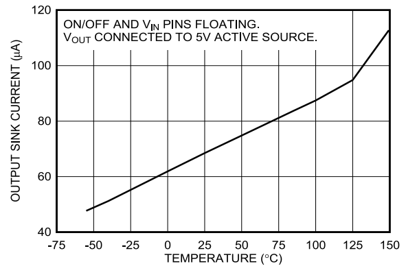
Figure 5-44. Output Reverse Leakage vs Temperature (New Chip)
