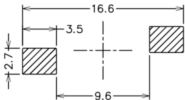
Soldering patterns
