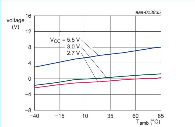
Fig 20. Switch output to input offset voltage versus ambient temperature
