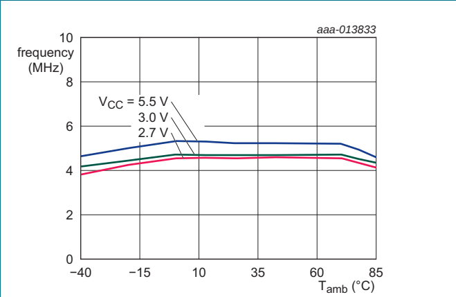
Fig 18. Post detection amplifier -3 dB bandwidth versus ambient temperature
