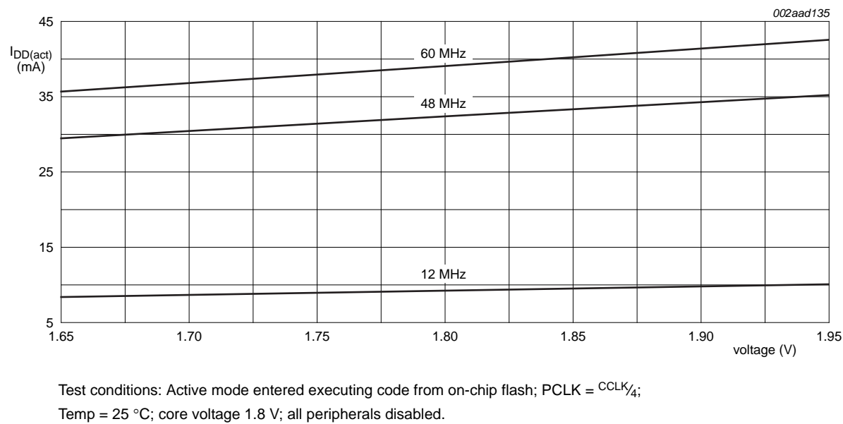
Fig 13. Typical LPC2109/01, LPC2119/01, and LPC2129/01 I_{DD(act)} measured at different voltages
