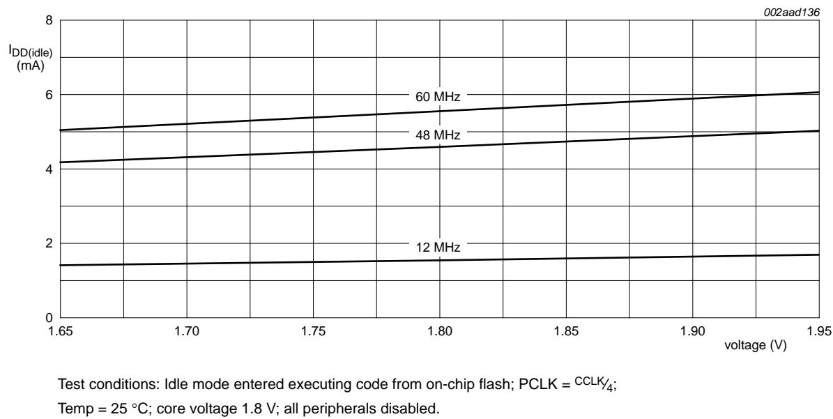
Fig 14. Typical LPC2109/01, LPC2119/01, and LPC2129/01 I_{DD(idle)} measured at different voltages
