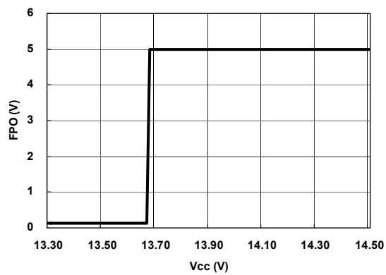
Figure 8. +12V OVP Voltage
