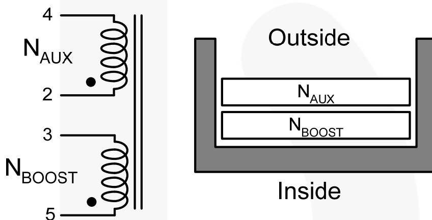
Figure 5. Boost Inductor used in this FAN9611 / 12 Evaluation Board
