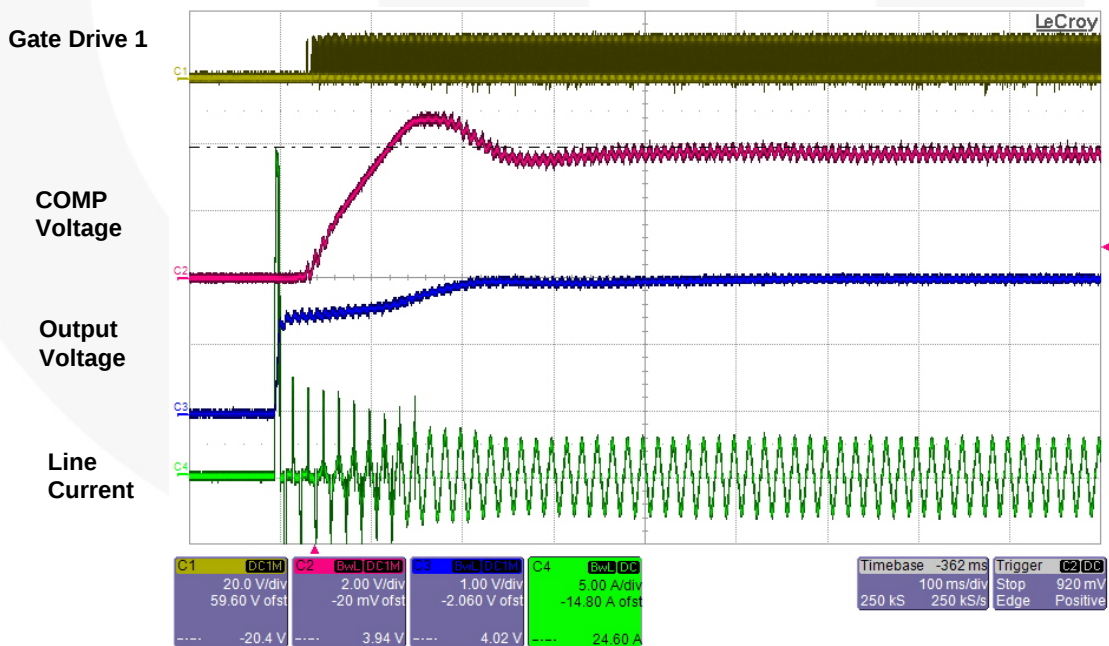
Figure 17. No-Load Startup at 230 V AC
