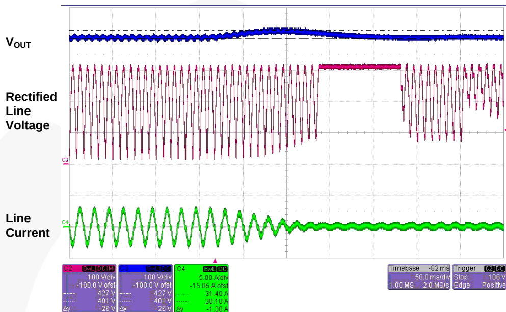
Figure 25. Load Transient Response at 230 V AC (Full Load → No Load)
