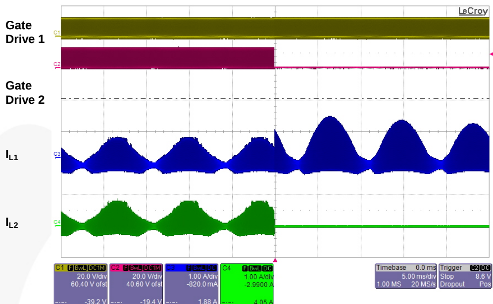
Figure 31. Phase-Shedding Operation
