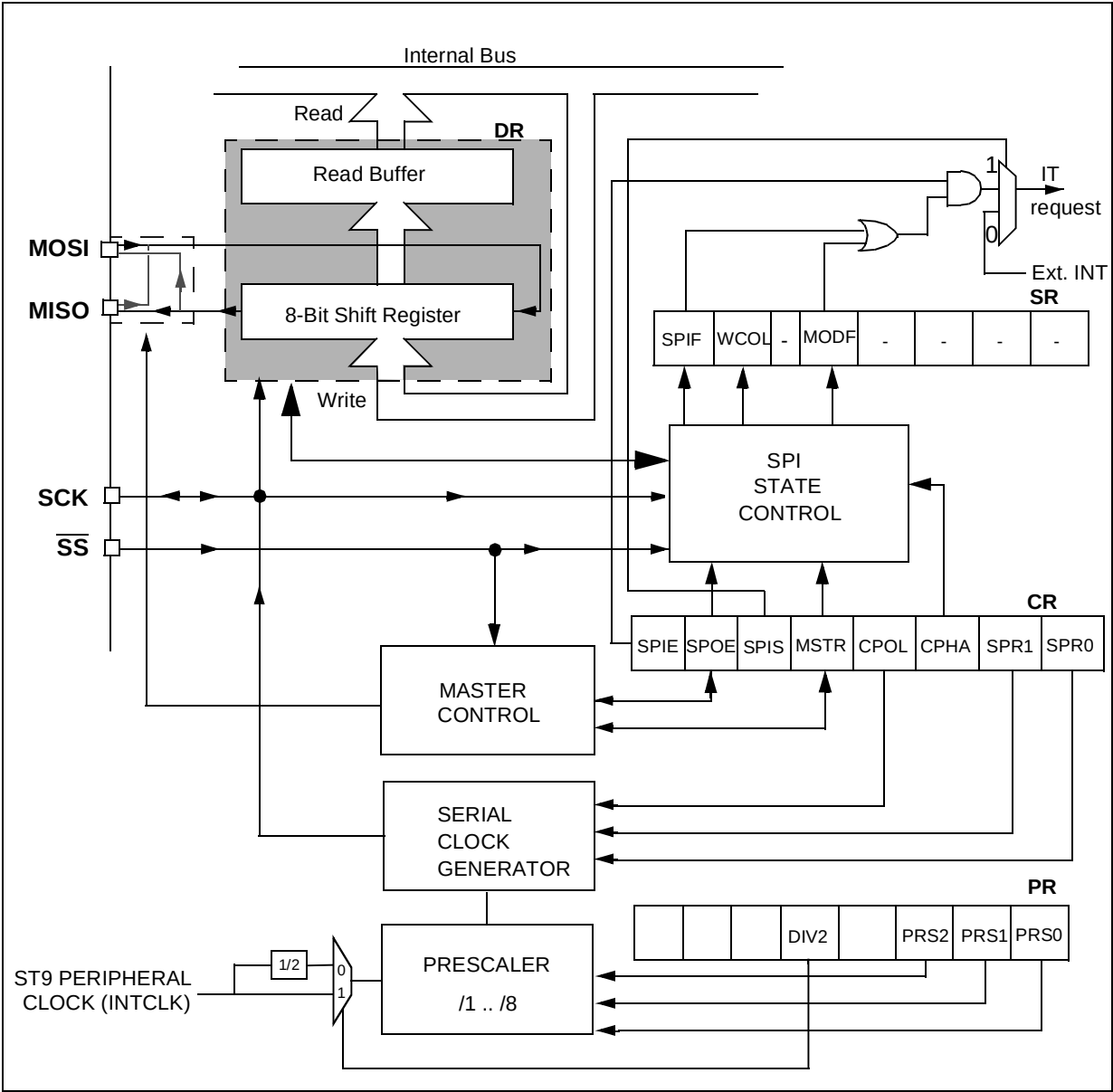
Figure 73. Serial Peripheral Interface Block Diagram
