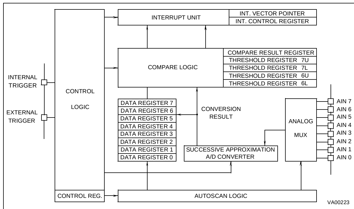
Figure 78. Block Diagram
