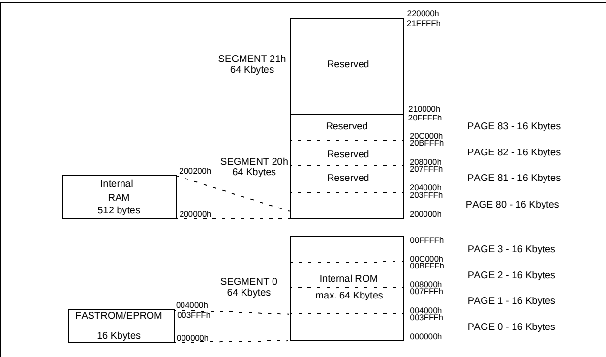
Figure 2. Memory Map
