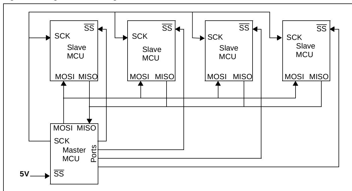
Figure 77. Single Master Configuration
