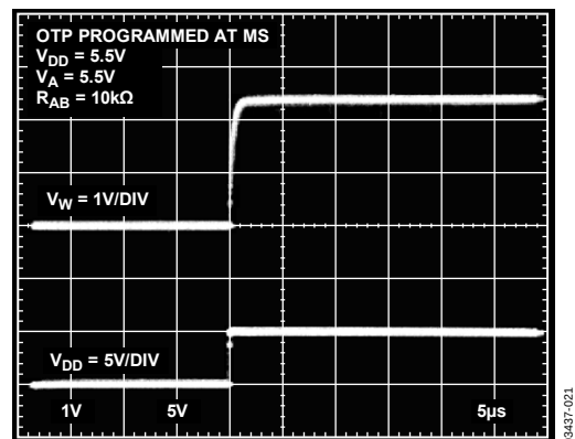
Figure 22. Power-Up Settling Time After Fuses Blown
