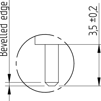
DETAIL B (5:1)
