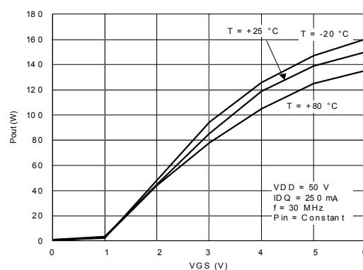
Figure 23. Output power vs. gate-source voltage
