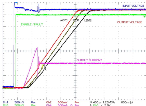
Figure 13. V_{OUT} ramp-up vs. enable
