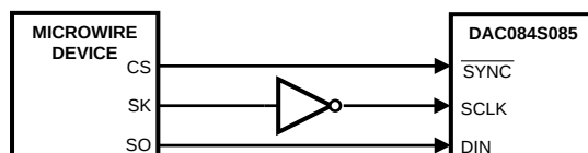
Figure 39. Microwire Interface
