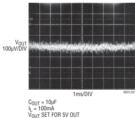
10Hz to 100kHz Output Noise C_{BYP} = 0.01µF
