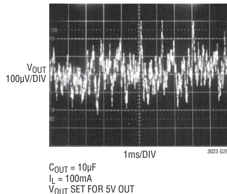
10Hz to 100kHz Output Noise C_{BYP} = 100pF
