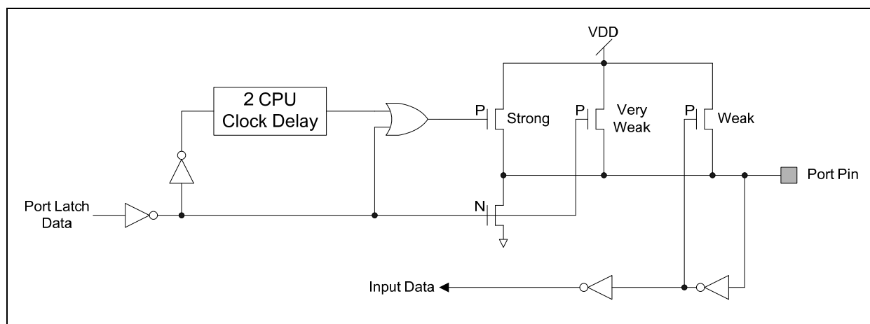
Figure 18-1: Quasi-Bidirectional Output
