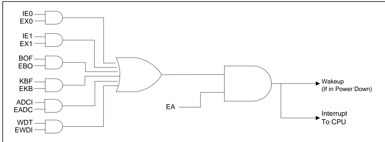
Figure 12-1: Interrupt Sources that can wake up from Power Down Mode
