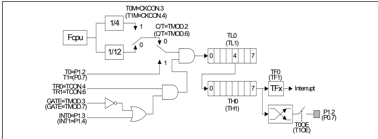
Figure 13-1: Timer/Counters 0 & 1 in Mode 0
