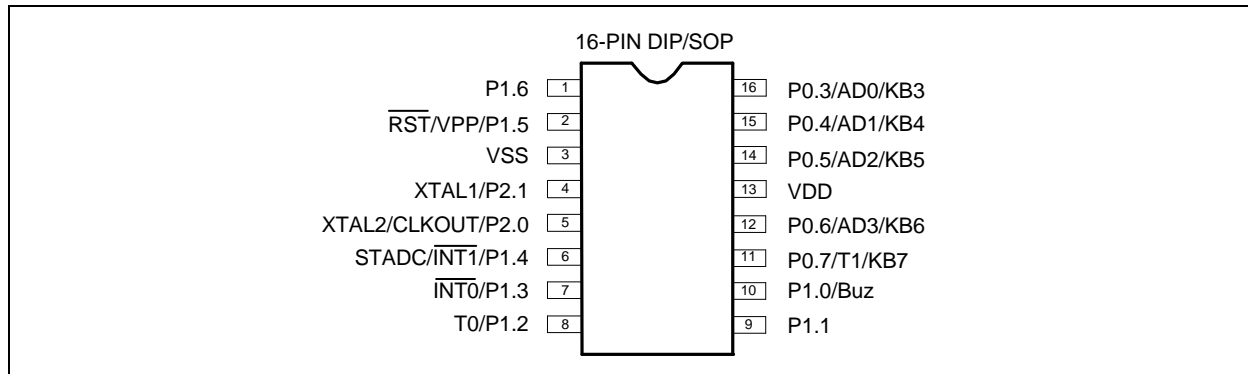
Figure 4-1: Pin Configuration
