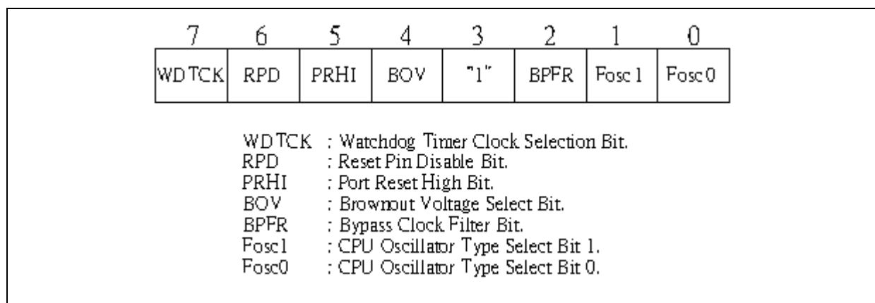
Figure 24-1: Config0 register bits
