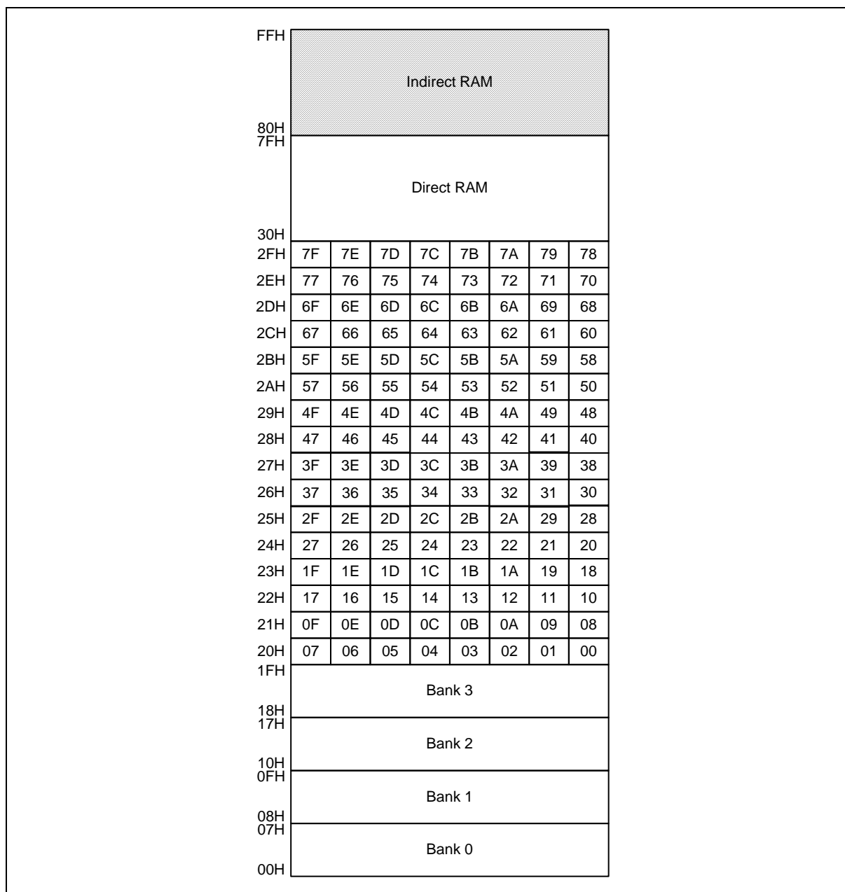
Figure 7-3: Scratch pad RAM
