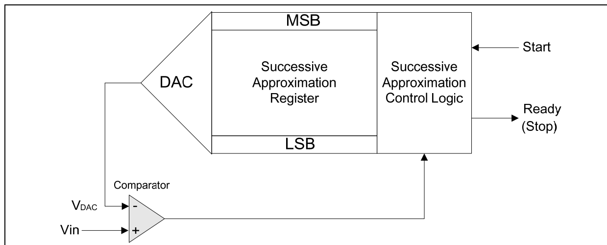
Figure 22-1: Successive Approximation ADC
