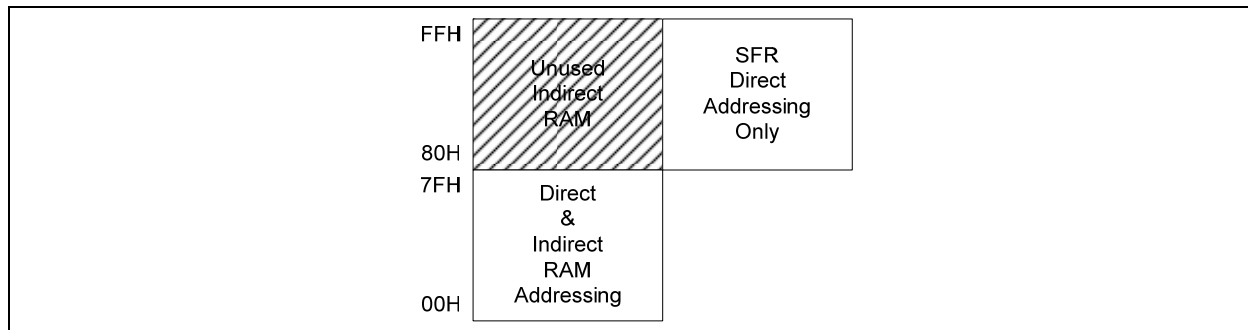
Figure 7-2: RAM and SFR memory map
