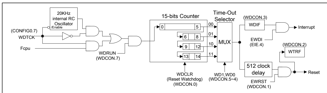
Figure 15-1: Watchdog Timer
