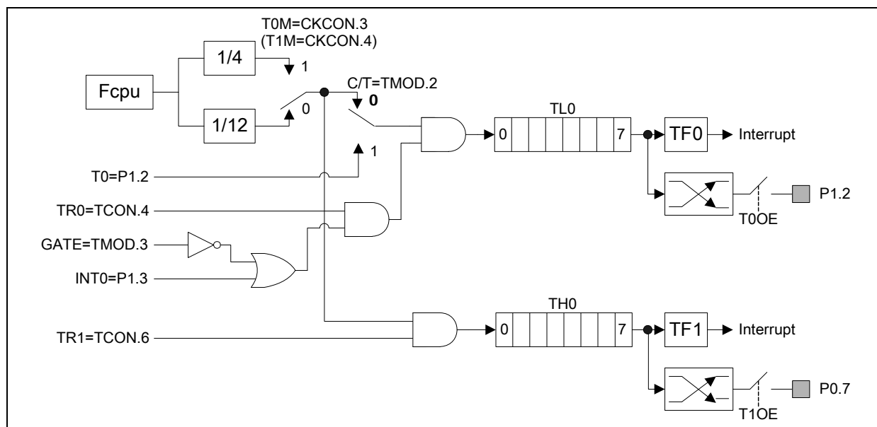
Figure 13-4: Timer/Counter Mode 3
