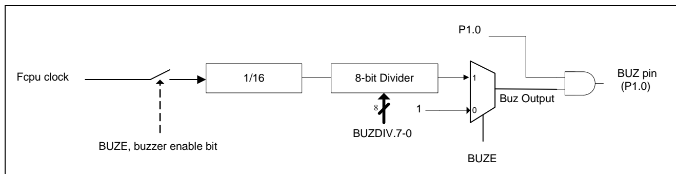
Figure 20-1: Square wave output
