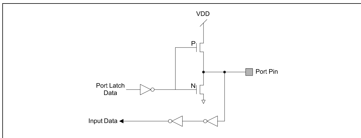
Figure 18-3: Push-Pull Output
