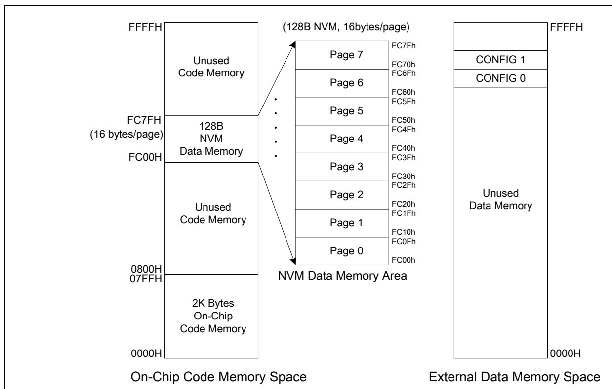
Figure 7-1: Memory map
