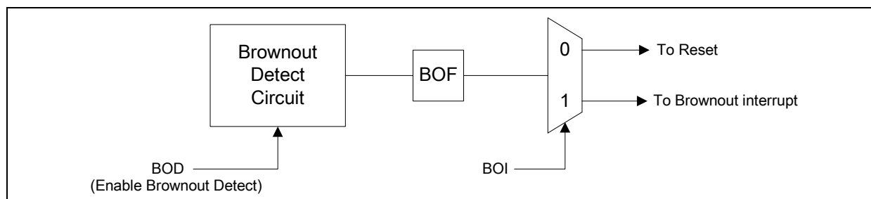
Figure 21-1: Brownout Detect Block
