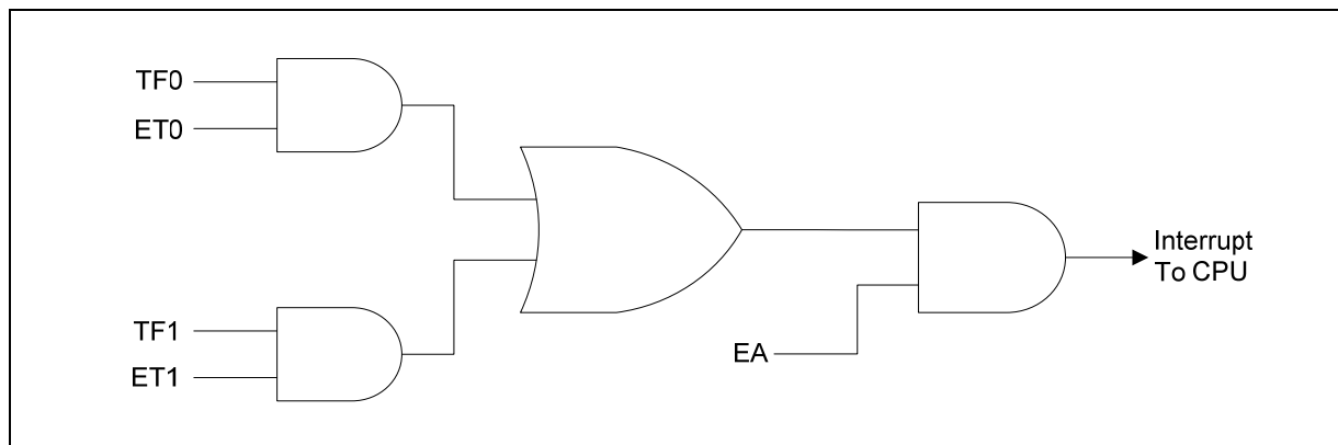
Figure 12-2: Interrupt Sources that cannot wake up from Power-down Mode
