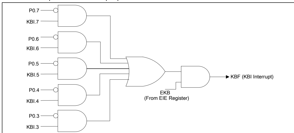
Figure 17-1: Keyboard Interrupt
