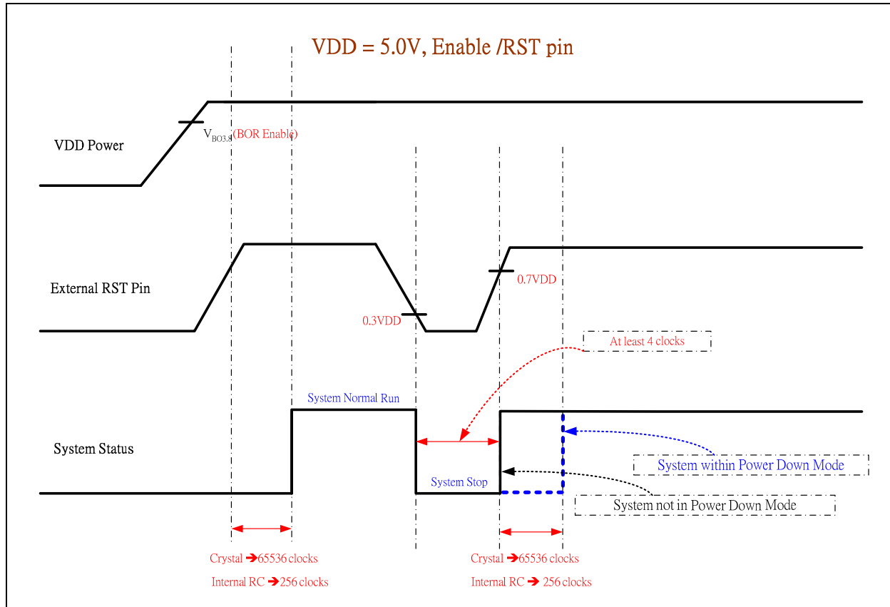
Figure 11-2: Reset and Vdd monitor timing diagram, enable /RST pin.
