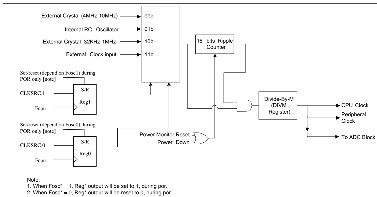
Figure 19-1: Oscillator
