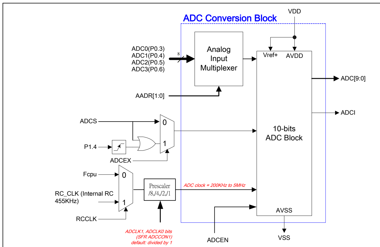
Figure 22-2: The ADC Block Diagram
