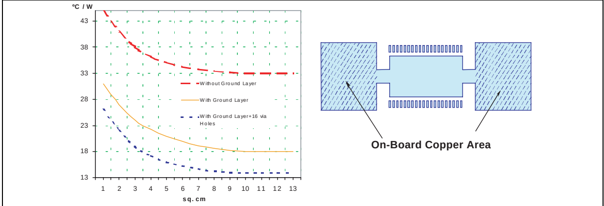
Figure 18. PowerSO20 Junction-Ambient thermal resistance versus on-board copper area.
