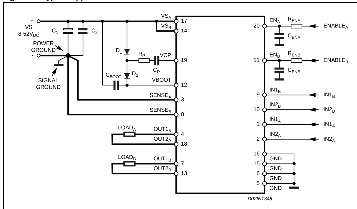
Figure 11. Typical Application
