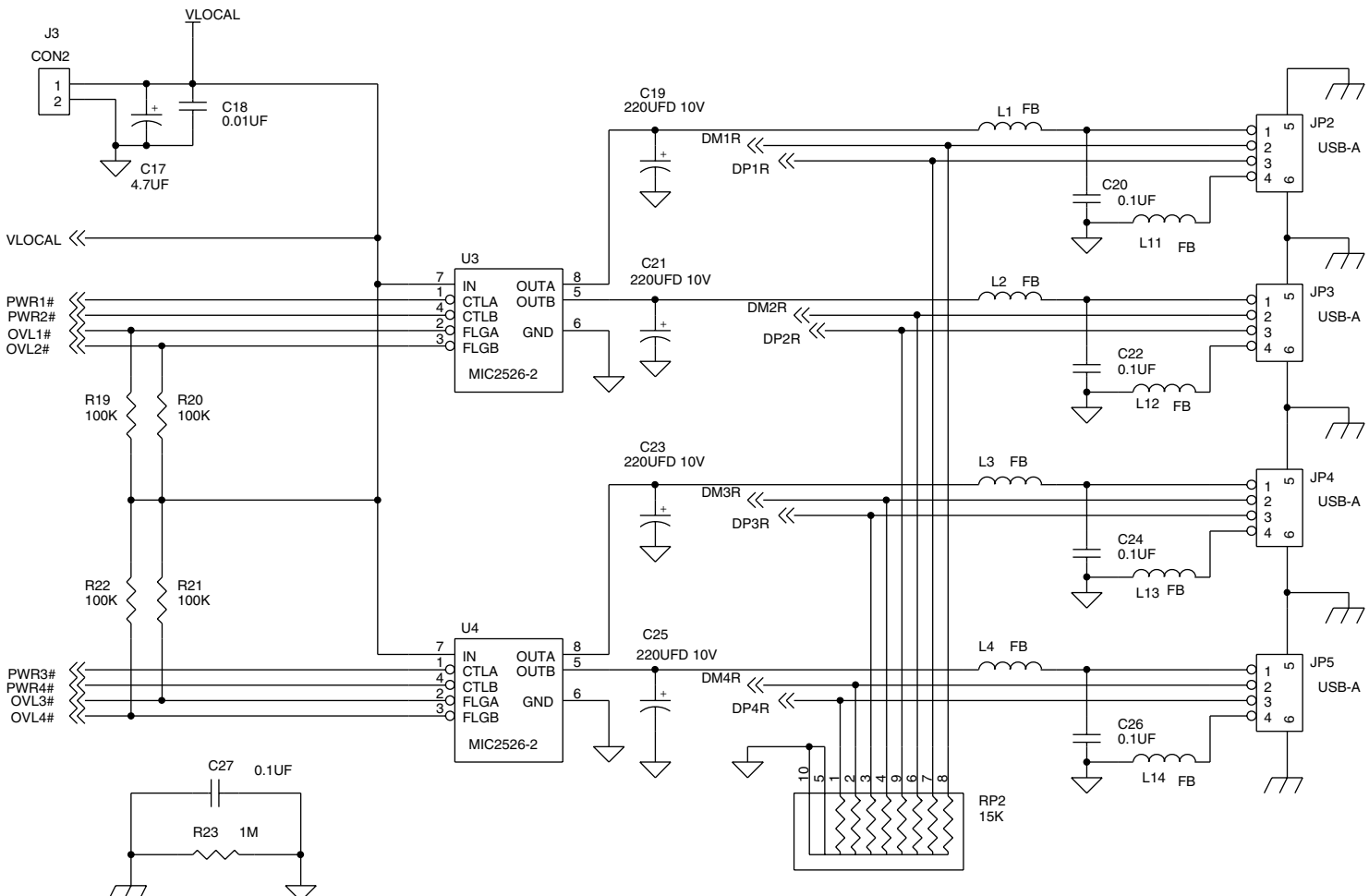
Figure 14. AT43312A Self-powered USB Hub
