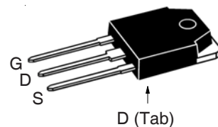
TO-247 (IXFH)
