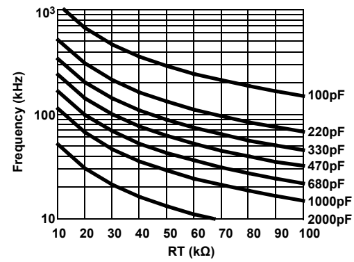
Figure 6. Resistance for CT Capacitor Values Given
