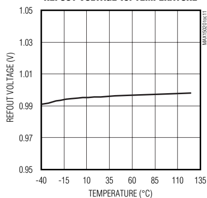
REFOUT VOLTAGE vs. TEMPERATURE
