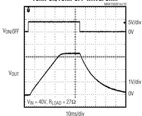
TURN-ON/TURN-OFF WAVEFORM
