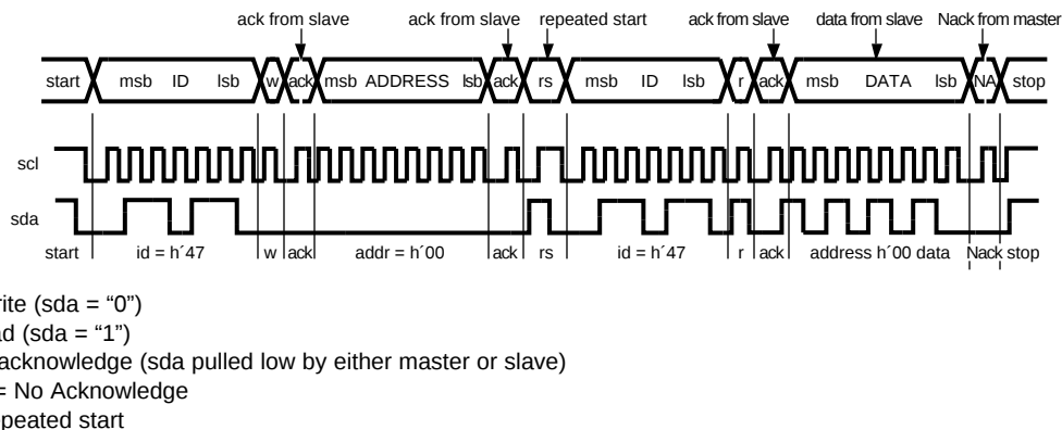
Figure 9. LP3947 (Slave) Register Read
