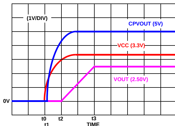
FIGURE 1. SOFT-START INTERVAL
