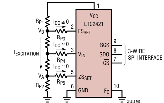
Figure 30. Half-Bridge Digitizer with Zero-Scale and Full-Scale Sense
