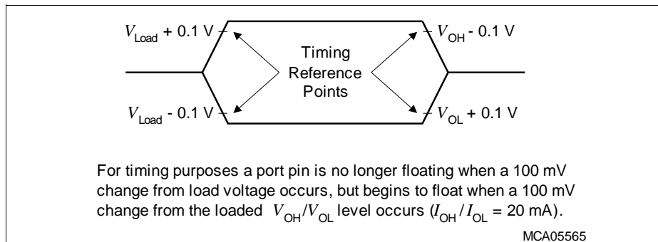
Figure 20 Floating Waveforms
