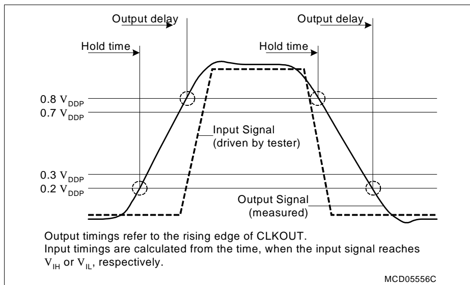
Figure 19 Input Output Waveforms
