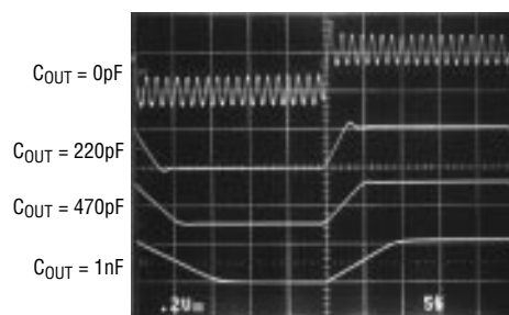
Small-Signal Response
