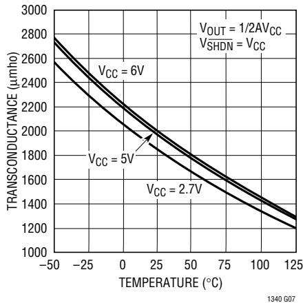
Transconductance vs Temperature
