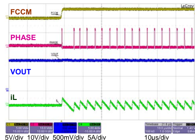
Figure 19: DCM/FCCM Transition
