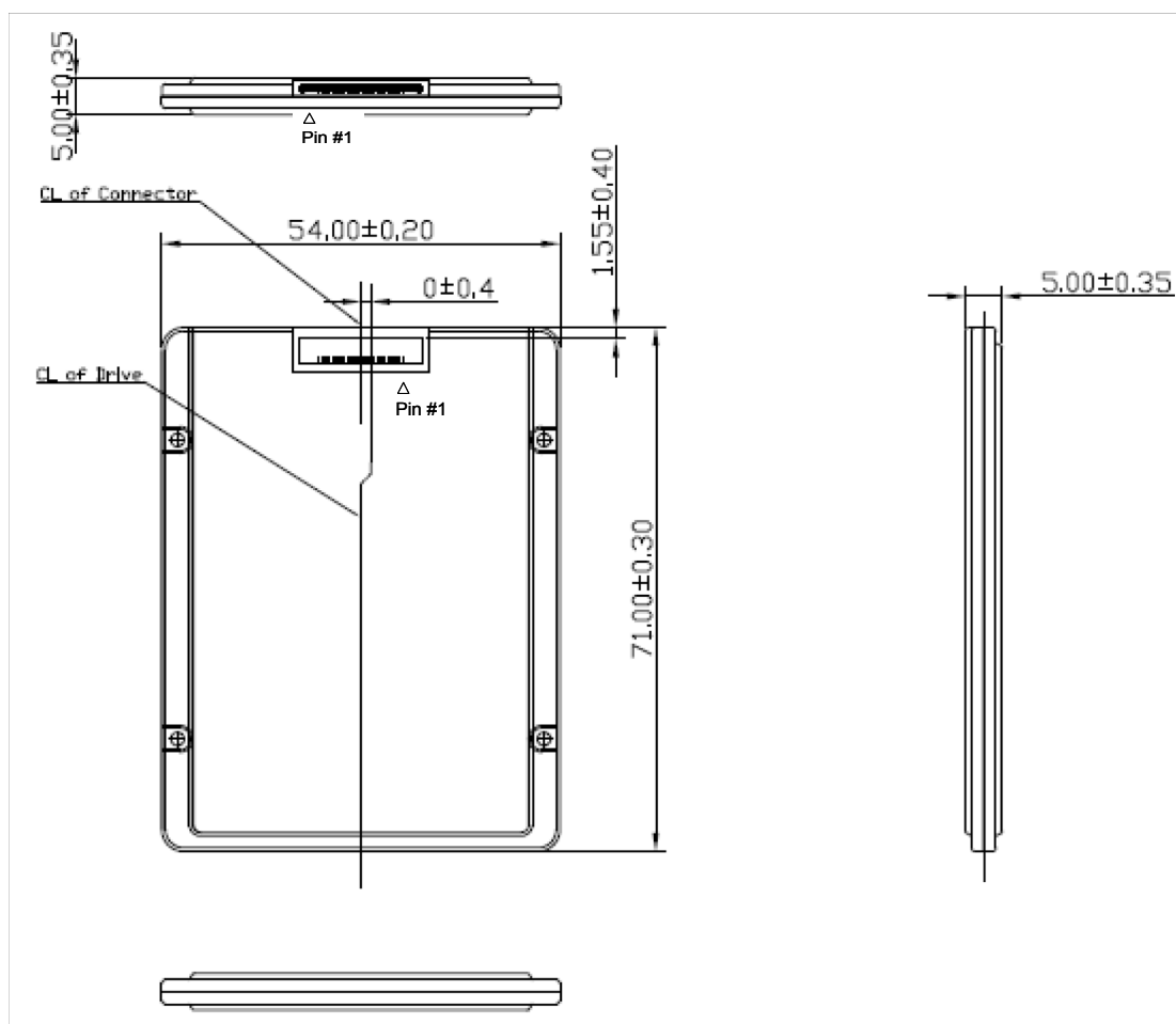
Figure 2-1. Physical dimension
