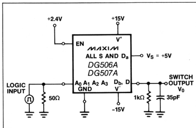
Figure 3. Break-Before-Make
